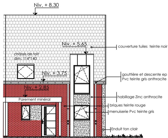
Façade Principale
